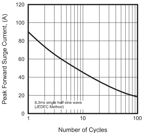
Fig.4 - Maximum Non-Repetitive Peak Forward Surge Current
